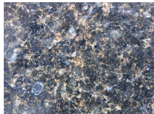
Charnockita
